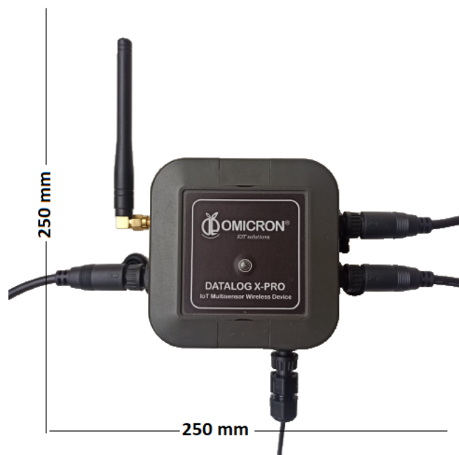
Figure 3-1 Recommended free space around the Datalog X-PRO
